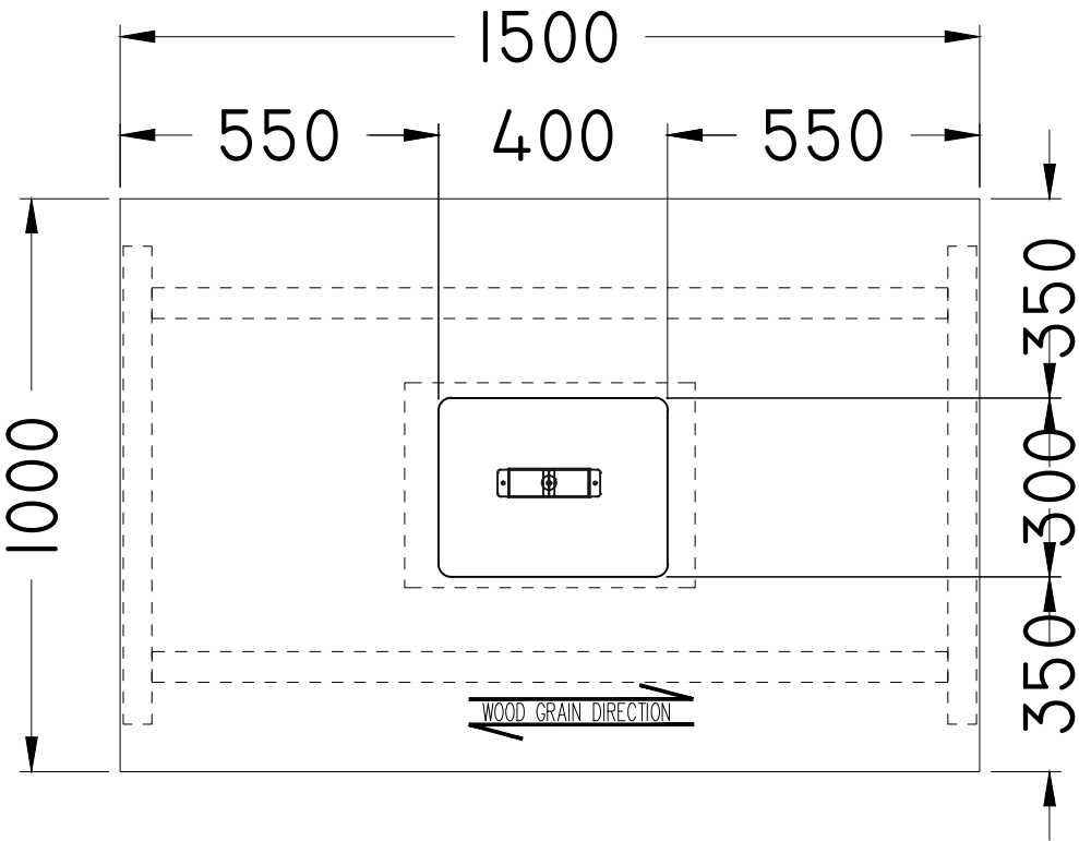
PLAN VIEW 1:20 ON A3
