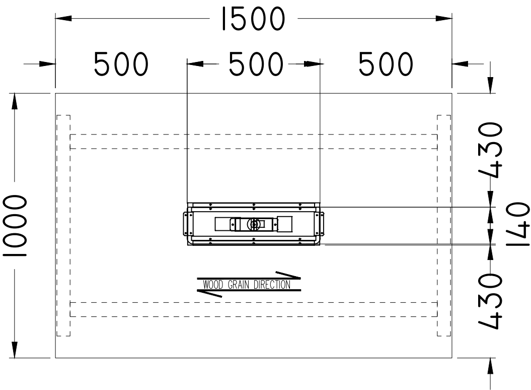
PLAN VIEW 1:20 ON A3
