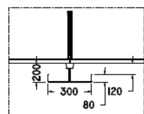
SPECIAL CABLE TRAY FOR LEXICON BENCH
