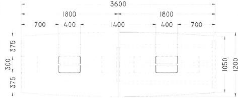
SIDE VIEW
