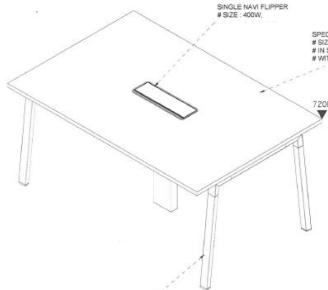
SPECIAL LEXICON BENCH(UNDERSTRUCTURE) # SIZE : 1500W 1000D, # WITH ANGLED/ANGLED LEGS, # WITHOUT CABLE MANAGEMENT
