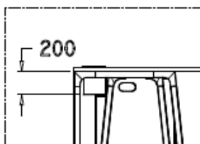
SPECIAL CABLE TRAY FOR LEXICON DESK
