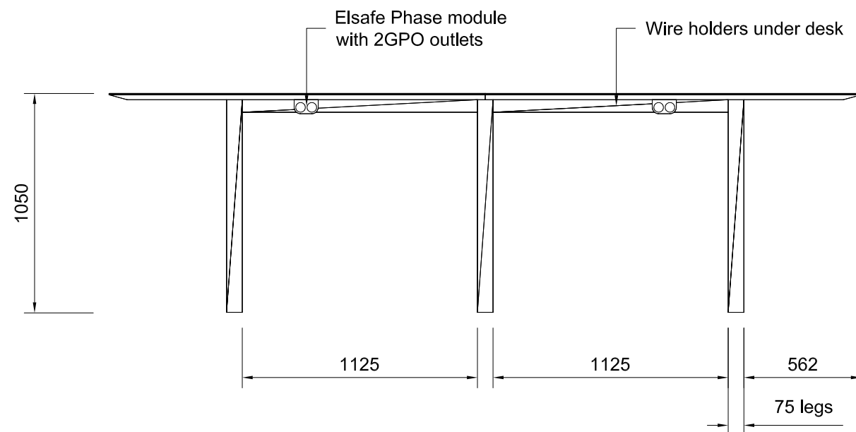
02 FRONT VIEW 1:25@A3
