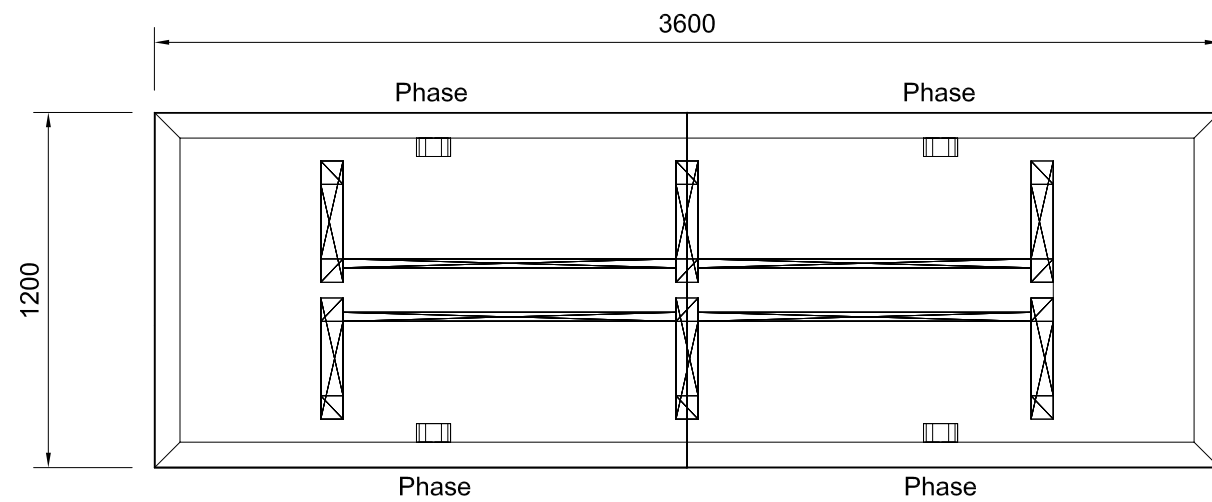
01 PLAN VIEW 1:25@A3
