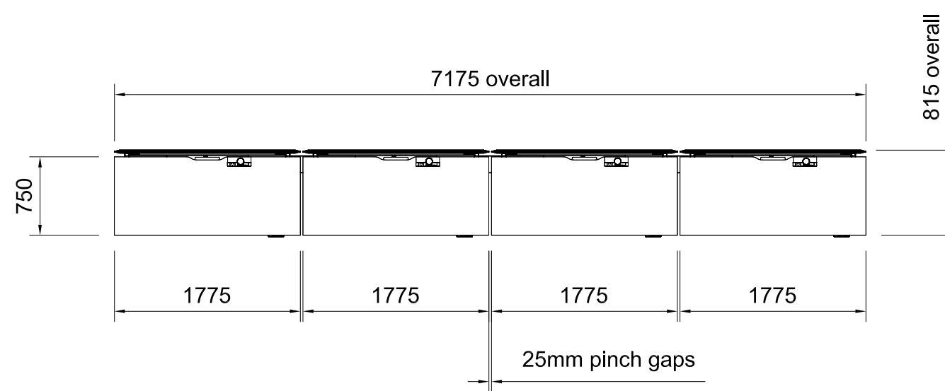
01 PLAN VIEW 1:50@A3
