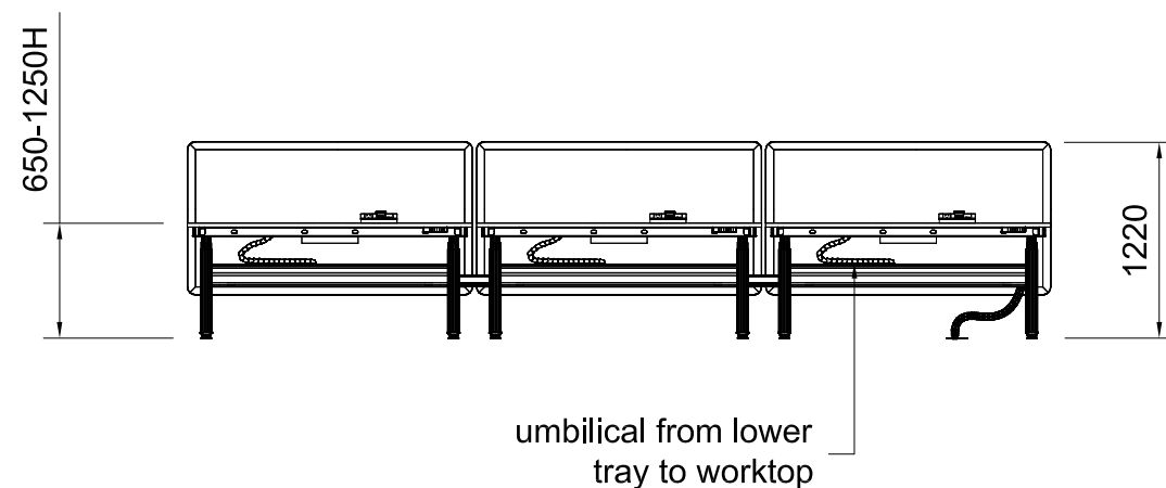
02 FRONT ELEVATION 1:50@A3
