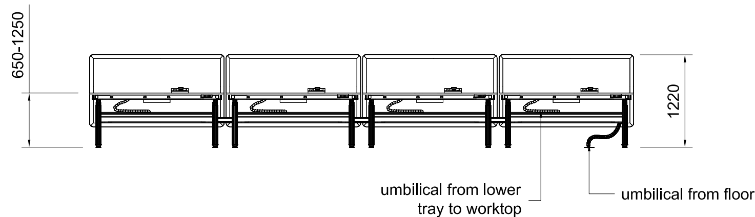
02 FRONT ELEVATION 1:50@A3
