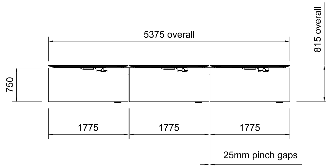
01 PLAN VIEW 1:50@A3
