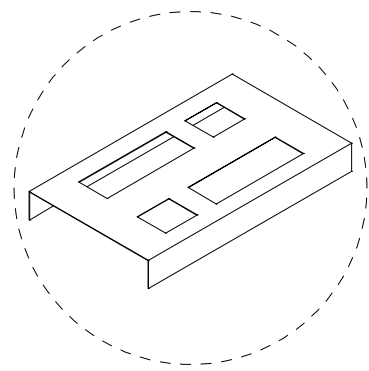
SPECIAL C CHANNEL # SIZE 600W 300D 60H # WITH CUT OUT AS ADVISED BY SALES
